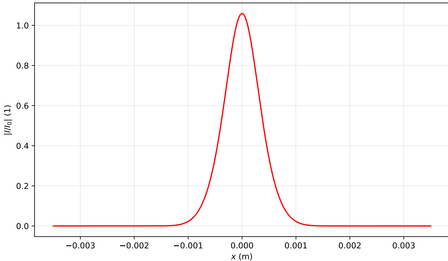
Intensity profile I(x, y = 0, z = 0.716)/I_0 , P_{in}=0.5P_{cr} , artificial time
